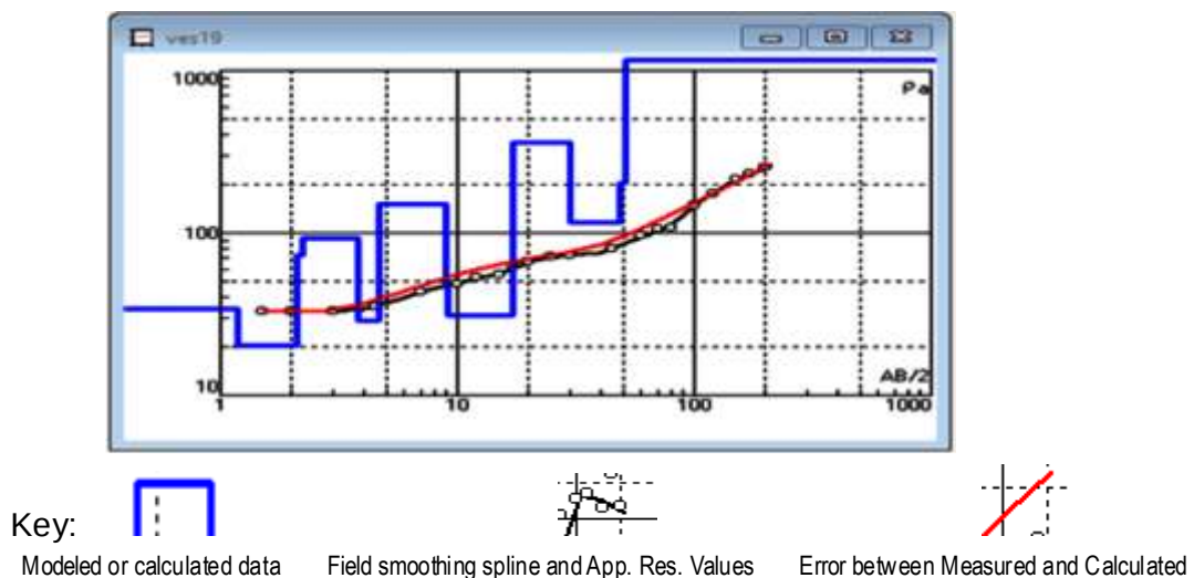
Figure 4. VES 19: Apparent Resistivity Curve Windows using the IPI2WIN software .
