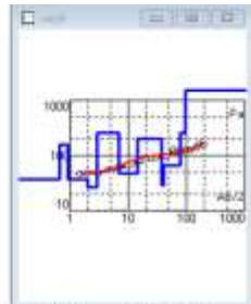
Apparent Resistivity Model Parameter Table and Curve Windows for VES Station No.9
